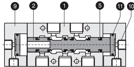
5/2 Double Pilot High Flow Valve
