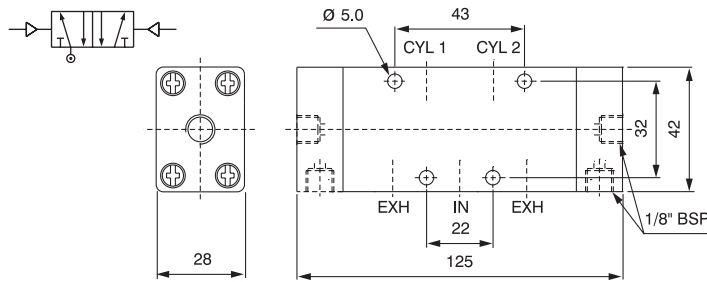
5/2 Double Pilot High Flow Valve
