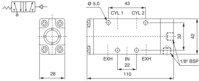
5/2 Single Pilot High Flow Valve
