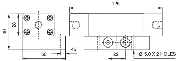
5/2 Double Pilot High Flow Valve ( Sub base )
