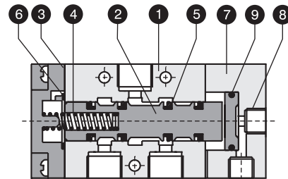
3/2 Single Pilot High Flow Valve
