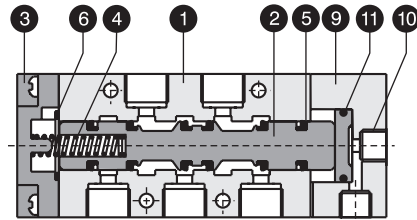
5/2 Single Pilot High Flow Valve
