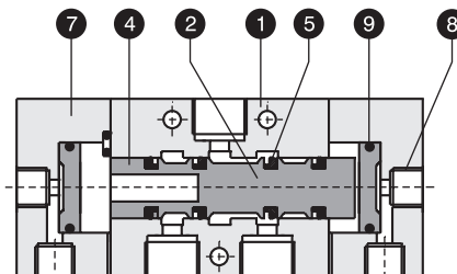
3/2 Double Pilot High Flow Valve
