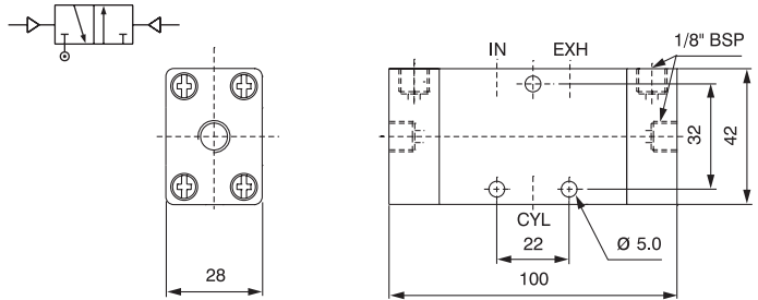
3/2 Single Pilot High Flow Valve
