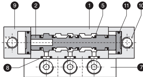
5/2 Double Pilot High Flow Valve ( Sub base )
