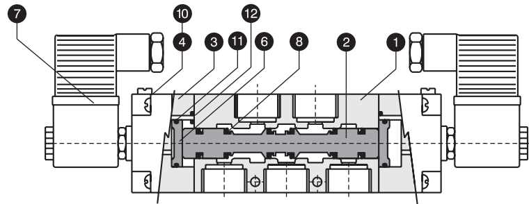
Double solenoid valve
