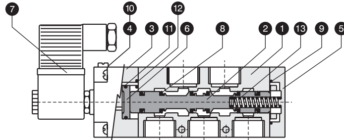
Single solenoid valve
